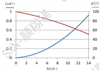
SMMS0518-1R0M
