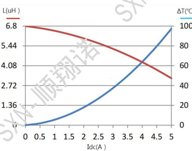
SMMS0518-6R8M
