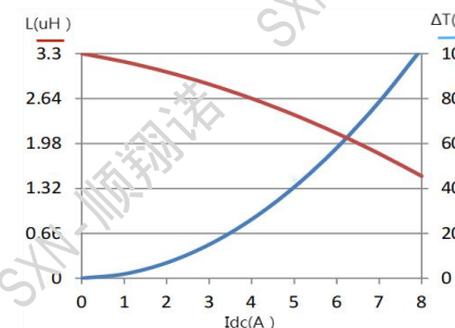
SMMS0518-3R3M
