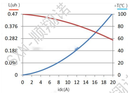
SMMS0518-R47M
