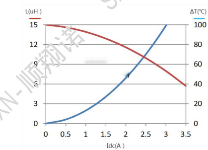
SMMS0518-150M
