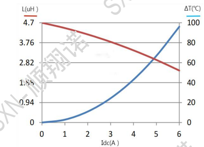
SMMS0518-4R7M
