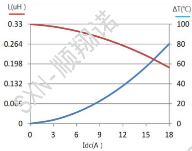
SMMS0518-R33M
