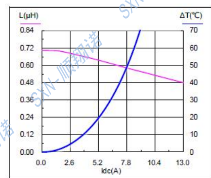
SMMS0420-R68M
