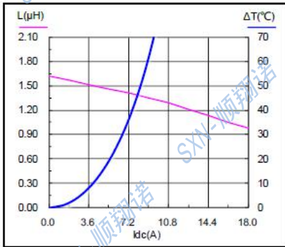
SMMS0624-1R5M
