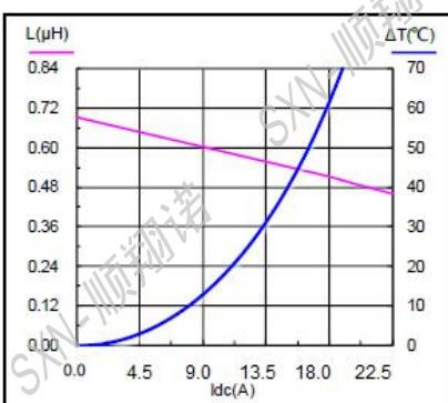
SMMS0624-R68M
