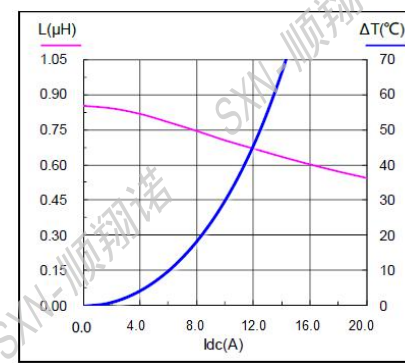
SMMS0624-R82M
