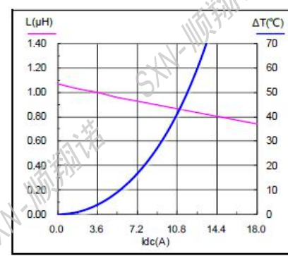
SMMS0624-1R0M
