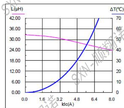
SMMS1360-330M
