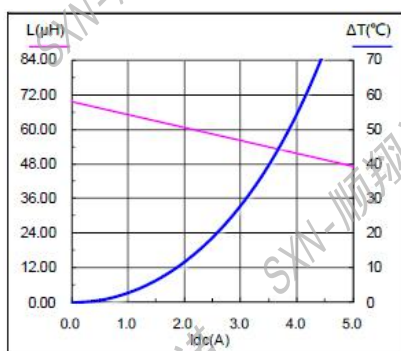
SMMS1360-680M
