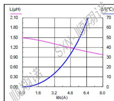
SMMS0520-1R5M
