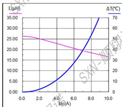
SMMS1360-270M
