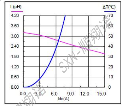
SMMS0624-3R3M
