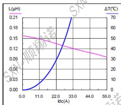
SMMS0630-R15M
