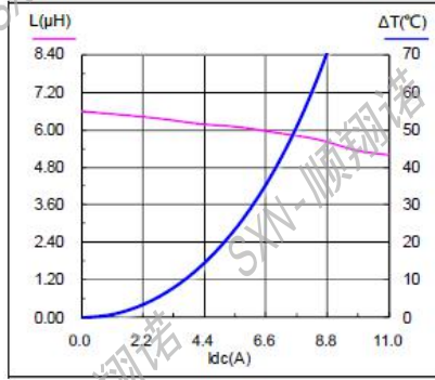
SMMS1040-6R8M
