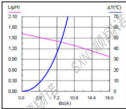
SMMS0624-1R5M
