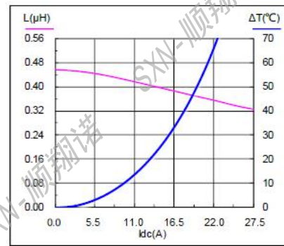
SMMS0624-1R0M
