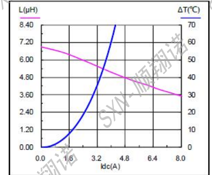
SMMS0624-6R8M
