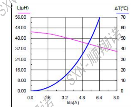
SMMS1360-470M
