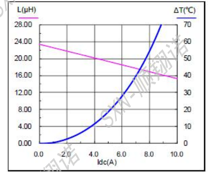
SMMS1360-220M
