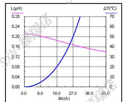
SMMS0630-R22M
