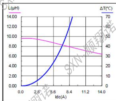
SMMS1050-100M
