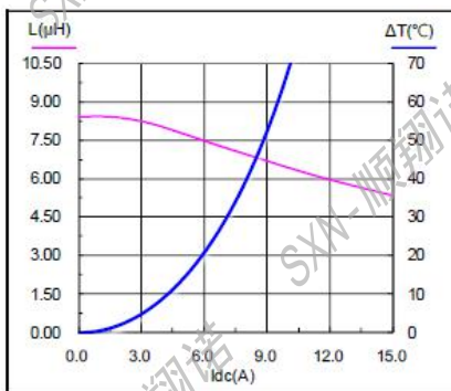
SMMS1050-8R2M
