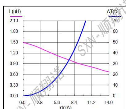
SMMS0530-1R5M
