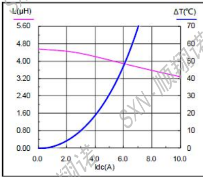
SMMS0630-4R7M
