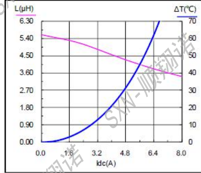
SMMS0630-5R6M
