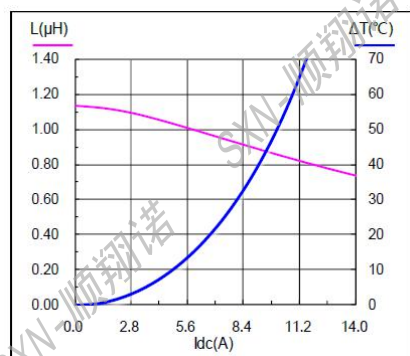
SMMS0530-1R0M
