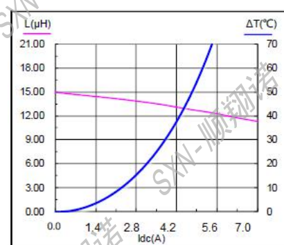
SMMS0650-150M
