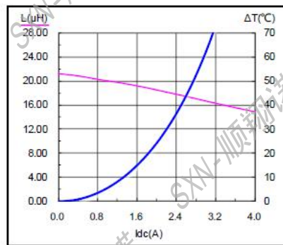
SMMS0630-220M
