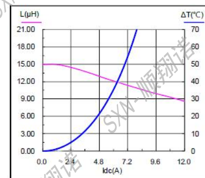
SMMS1050-150M
