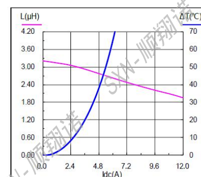
SMMS0530-3R3M
