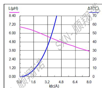
SMMS0530-6R8M
