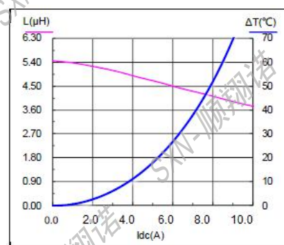
SMMS0650-5R6M
