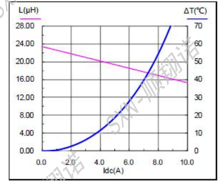
SMMS1360-220M
