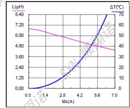
SMMS0630-6R8M
