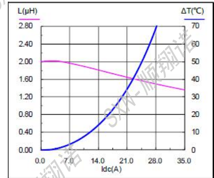
SMMS1360-2R2M
