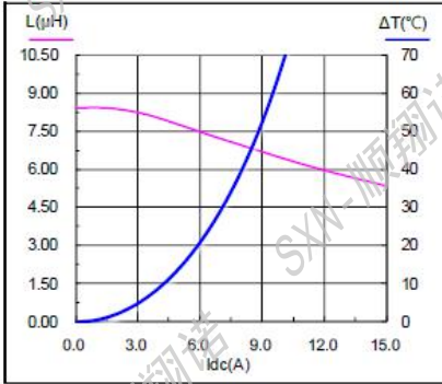
SMMS1050-8R2M
