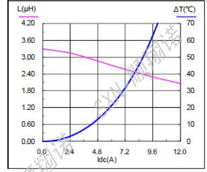
SMMS0630-3R3M
