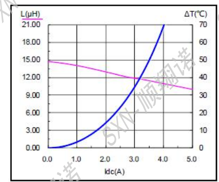
SMMS0630-150M
