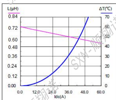
SMMS1360-R68M
