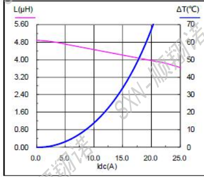
SMMS1360-4R7M
