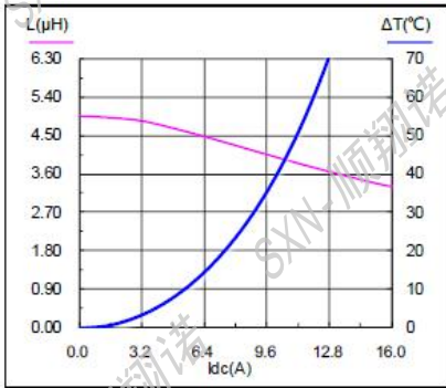
SMMS1040-4R7M
