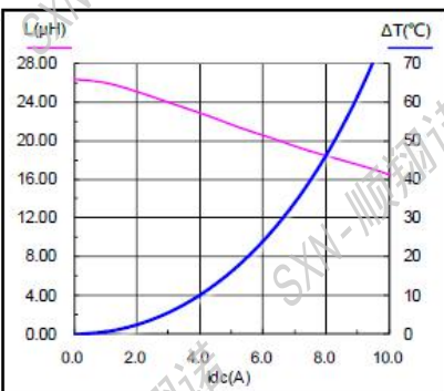
SMMS1350-220M
