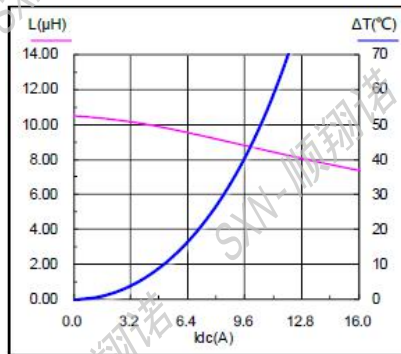
SMMS1350-100M
