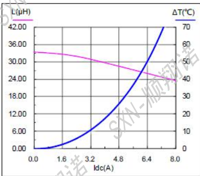
SMMS1350-330M
