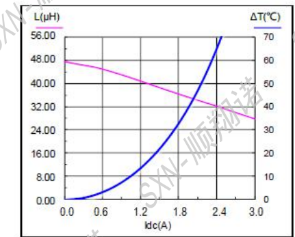
SMMS0630-470M
