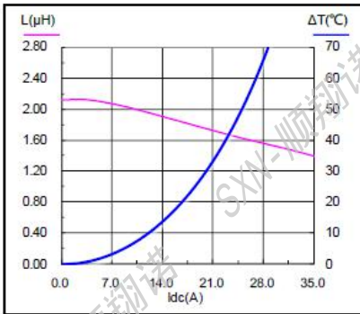
SMMS1350-2R2M
