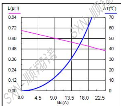
SMMS0624-R68M
