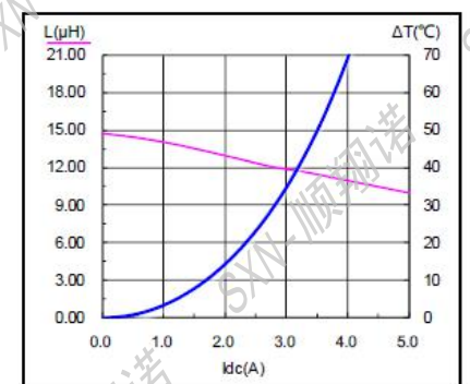
SMMS0630-150M
