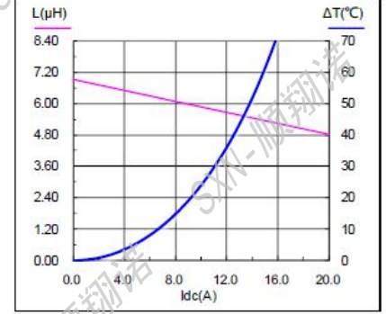
SMMS1360-6R8M
