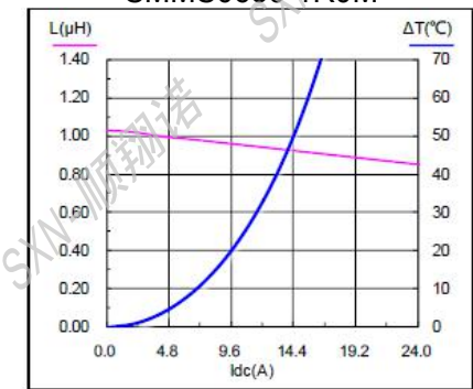
SMMS0630-1R0M
