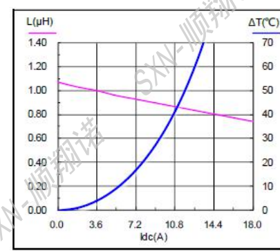
SMMS0624-1R0M
