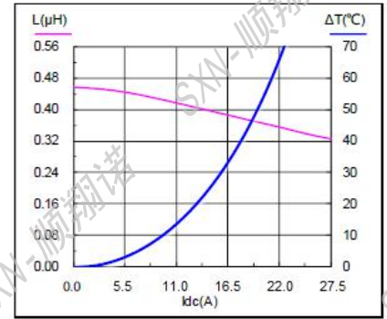
SMMS0624-1R0M
