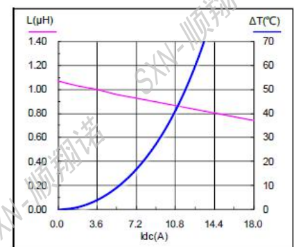
SMMS0624-1R0M
