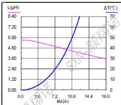
SMMS1050-5R6M
