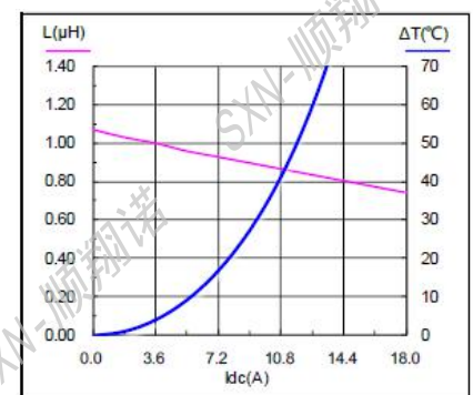
SMMS0624-1R0M
