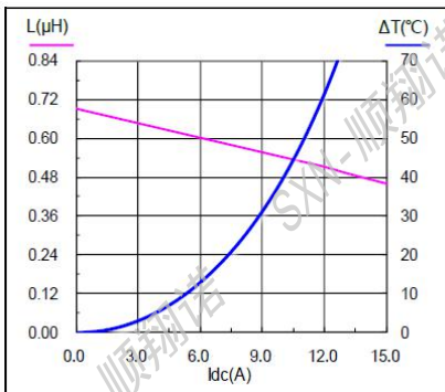
SMMS0530-R68M
