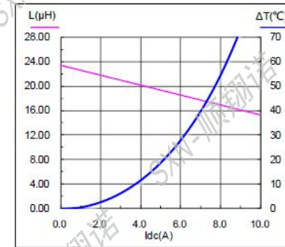
SMMS1360-220M
