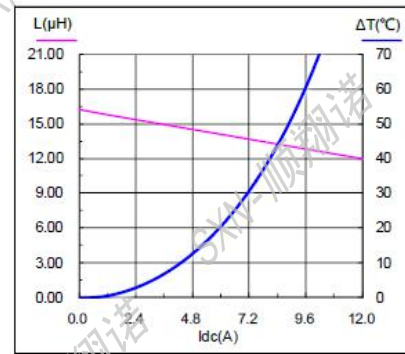
SMMS1350-150M
