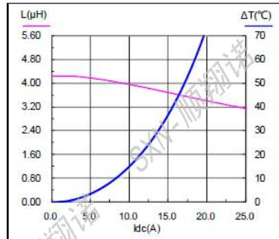
SMMS1350-4R7M
