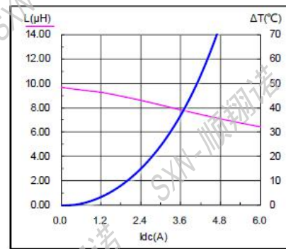
SMMS0630-100M
