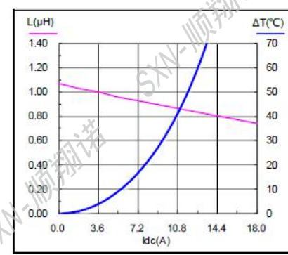
SMMS0624-1R0M
