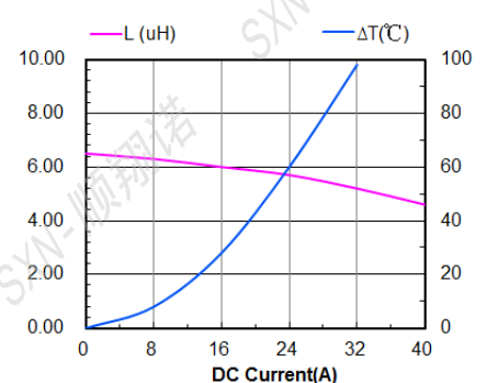
SMMS1770-6R8M
