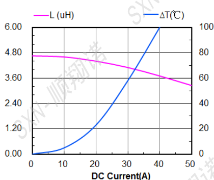
SMMS1770-4R7M
