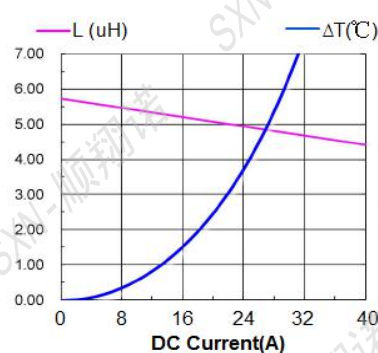
SMMS1770-5R6M
