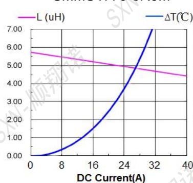
SMMS1770-5R6M
