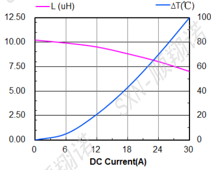
SMMS1770-330M
