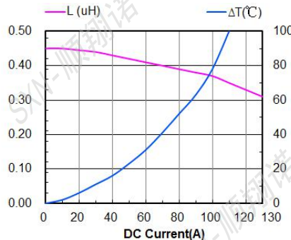
SMMS1770-R47M
