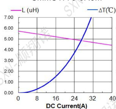
SMMS1770-5R6M
