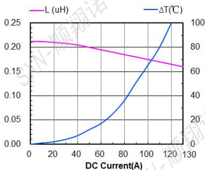
SMMS1770-R22M
