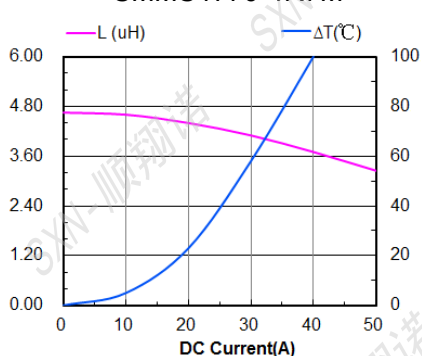
SMMS1770-4R7M
