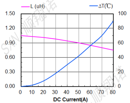
SMMS1770-1R0M
