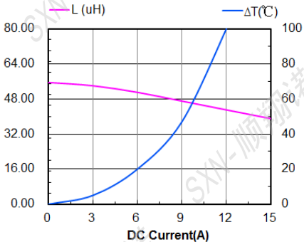
SMMS1770-560M
