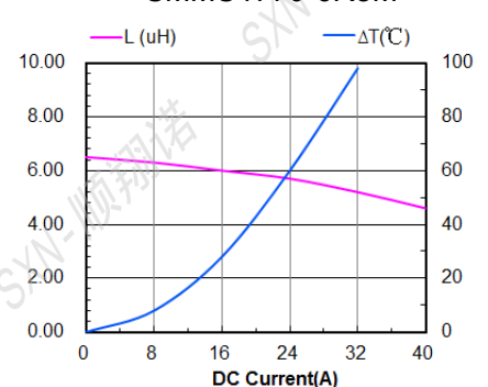
SMMS1770-6R8M
