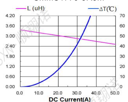
SMMS1770-6R8M
