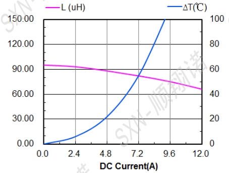
SMMS1770-101M
