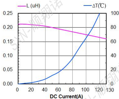
SMMS1770-R22M
