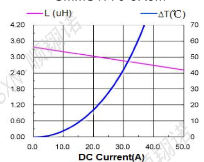
SMMS1770-6R8M
