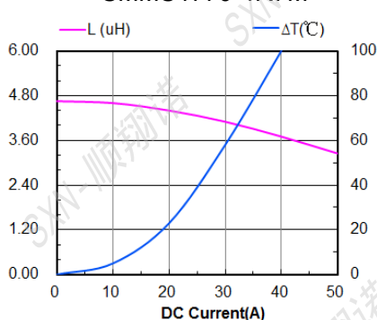
SMMS1770-4R7M
