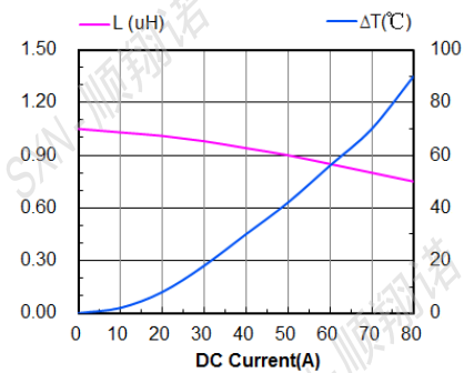
SMMS1770-1R0M
