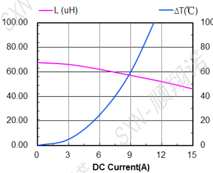
SMMS1770-680M
