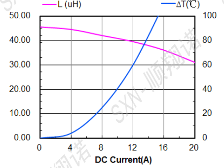
SMMS1770-101M
