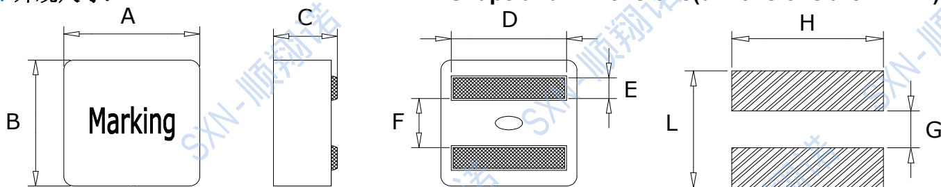
Recommended Land Pattern
