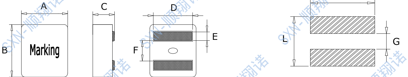
Recommended Land Pattern
