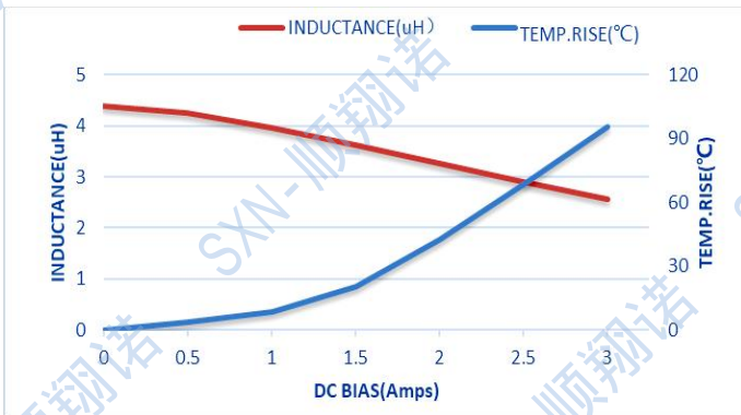
SMTC201610-4R7M
