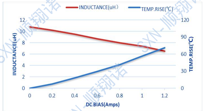
SMTC201610-100M
