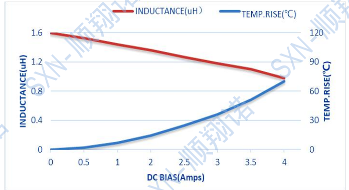
SMTC201610-1R5M
