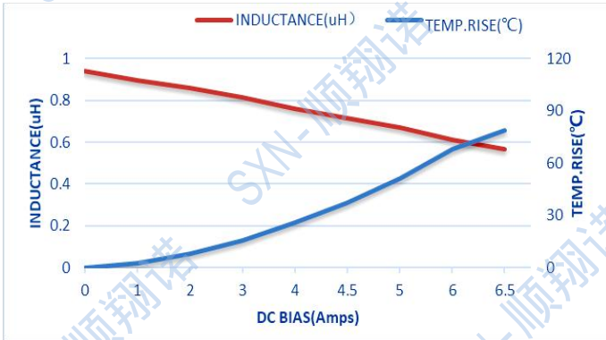
SMTC201610-1R0M
