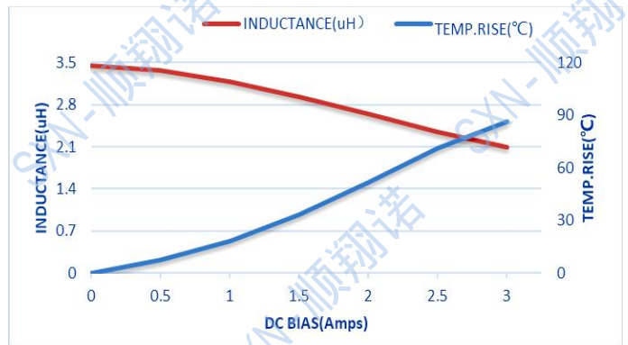
SMTC201610-3R3M
