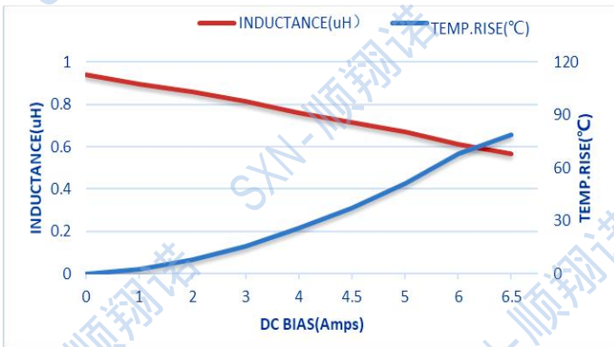
SMTC201610-1R0M
