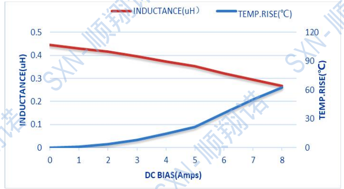
SMTC201610-R47M
