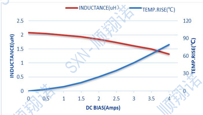
SMTC201610-2R2M
