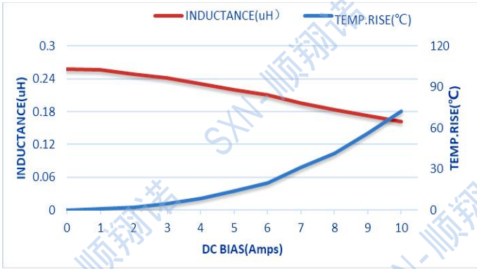
SMTC201610-R22M
