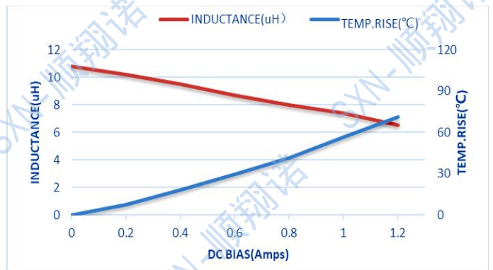
SMTC201610-100M
