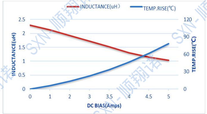
SMTC201612-2R2M
