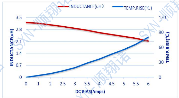
SMTC303020-3R3M
