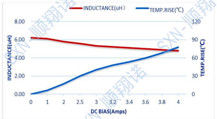
SMTC303020-6R8M
