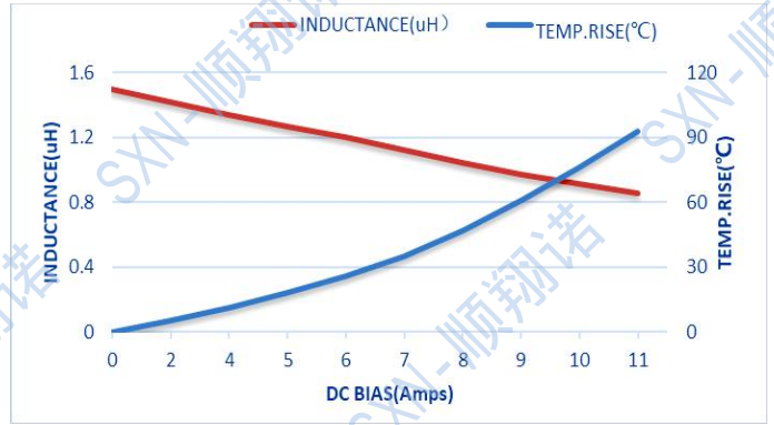
SMTC303020-1R5M
