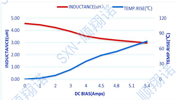
SMTC303020-4R7M
