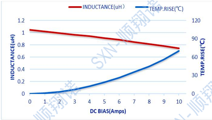
SMTC303020-1R0M
