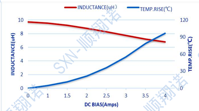
SMTC303020-100M
