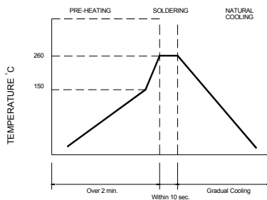
Wave Soldering Fig.2
