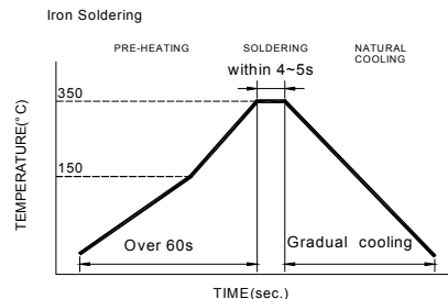
Iron Soldering times : 1 times max Fig.3
