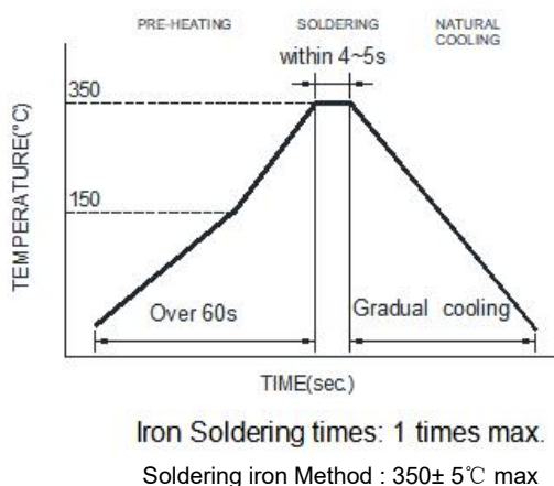
Fig.2 Iron Reflow
