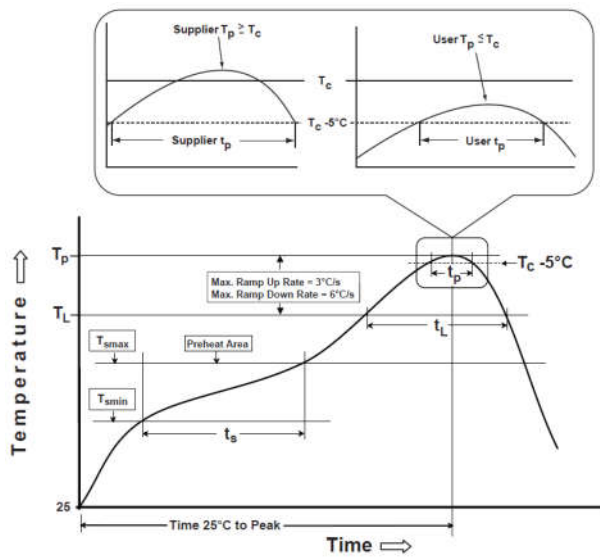
Fig.1 Soldering Reflow
