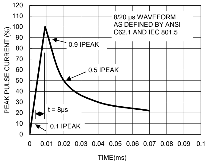
Fig.12 Pulse Waveform
