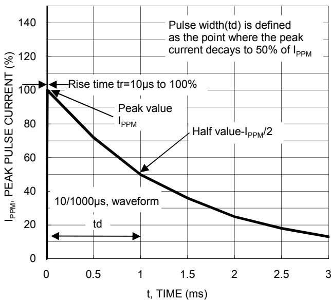
Fig.3 Clamping Power Pulse Waveform
