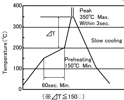
[Hand soldering] 【Recommended condition for Pb-free soldering】
