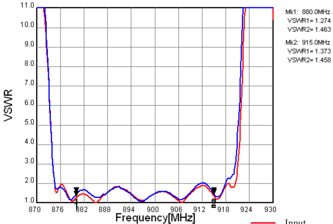
Fig.2 VSWR
