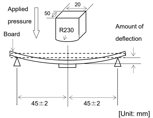
Fig. 4: Bending Strength Test Method
