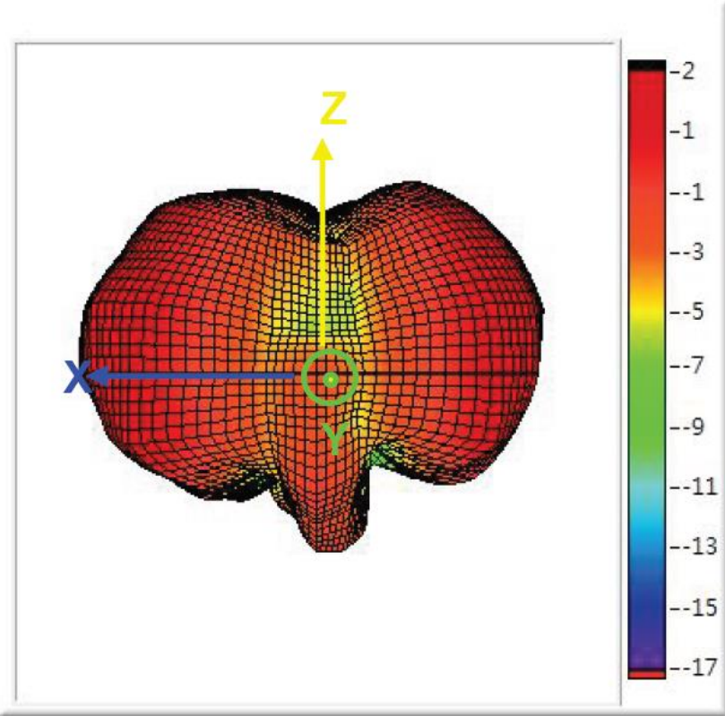
6.3 3D Gain pattern @ 5700 MHz
