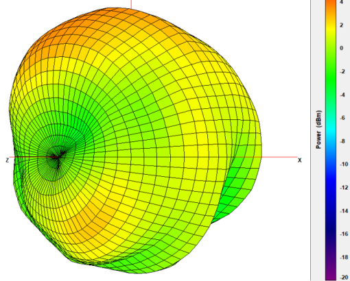
MIMO 1 – Free Space Azimuth = 0.0 Elevation = 0.0 Roll = -35.0
