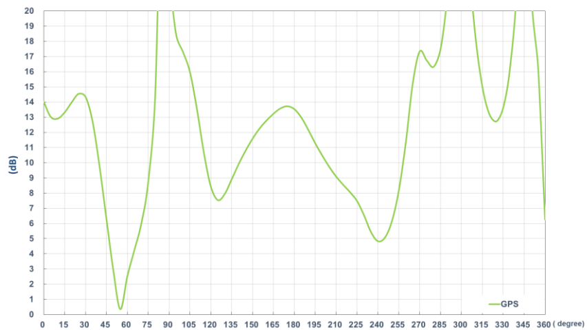
1575.42MHz
