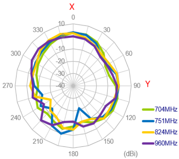
XY Plane
