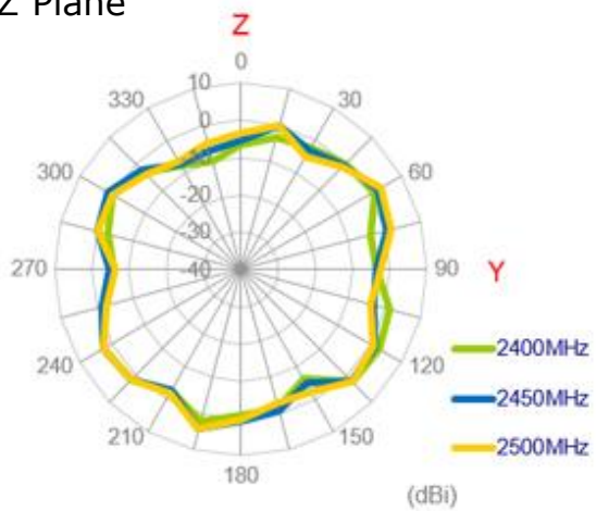
YZ Plane
