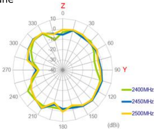
YZ Plane
