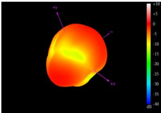
1575.42MHz
