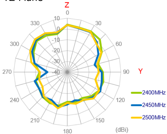
YZ Plane
