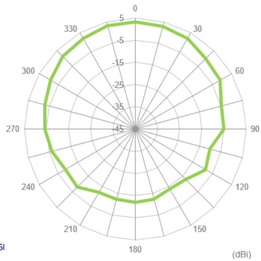
YZ Plane ( \phi=90^\circ , \Theta=0\sim 360^\circ )
