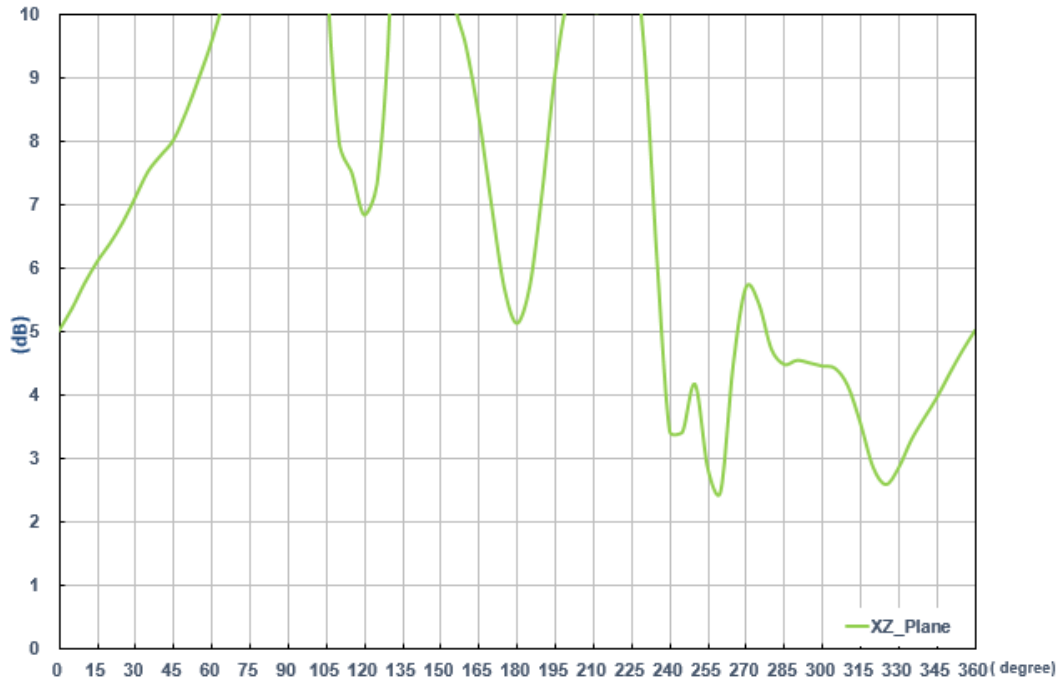
XZ Plane ( \phi=0^\circ , \Theta=-180\sim 180^\circ )
