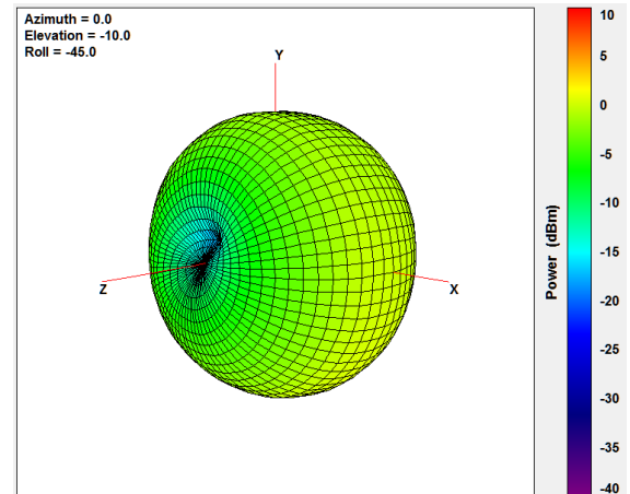
824MHz
