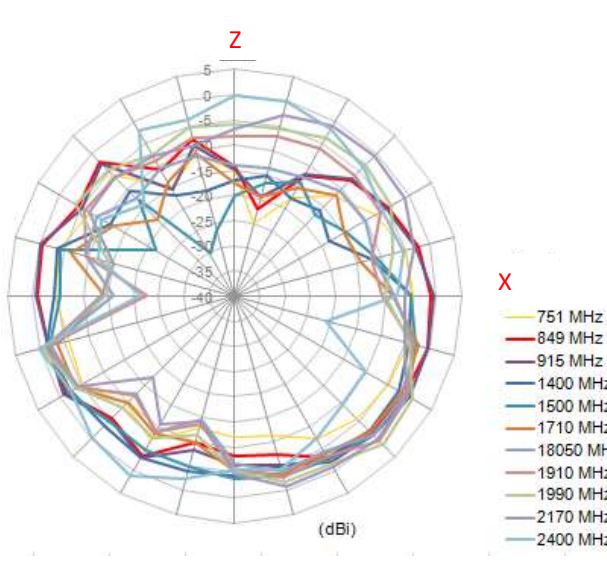
2D Radiation Pattern of the PA.700.J Antenna.
