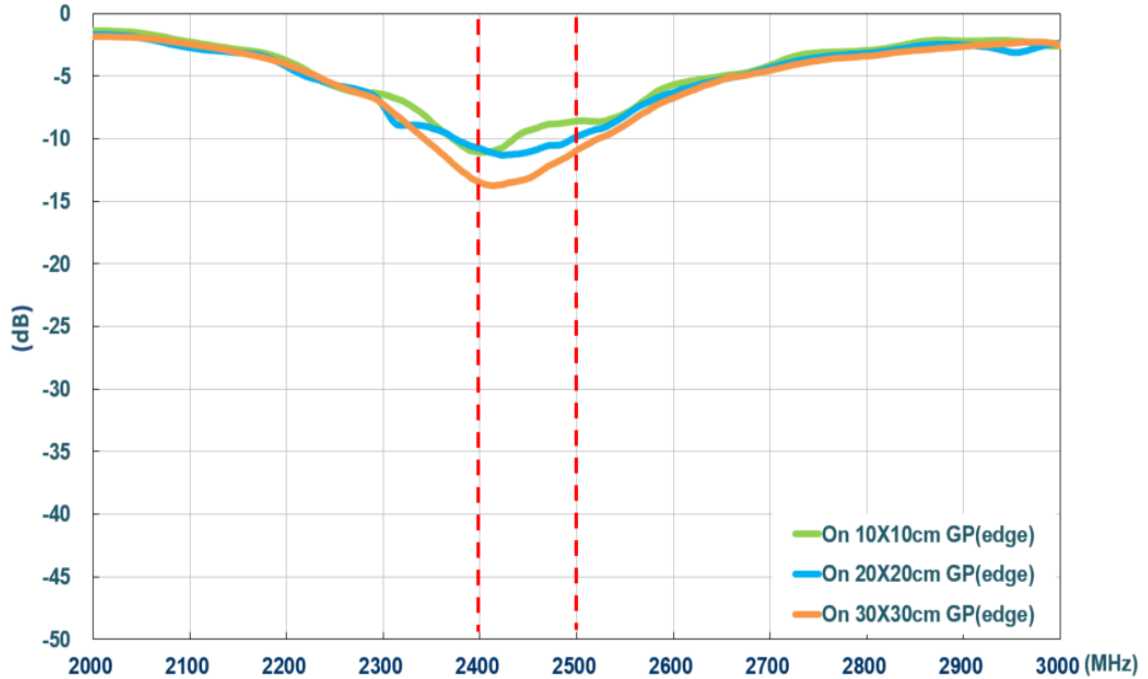
Figure 4. Return loss of WCM.01 on edge of different ground plane sizes
