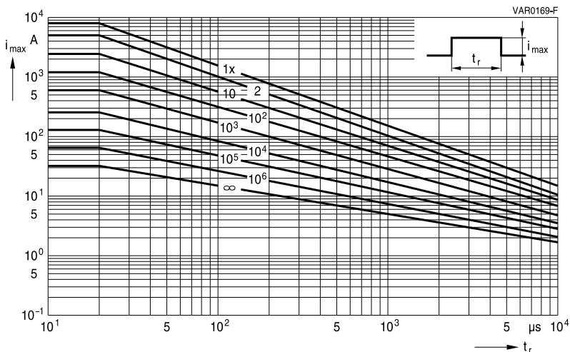
SIOV-S20K385 ... K460
