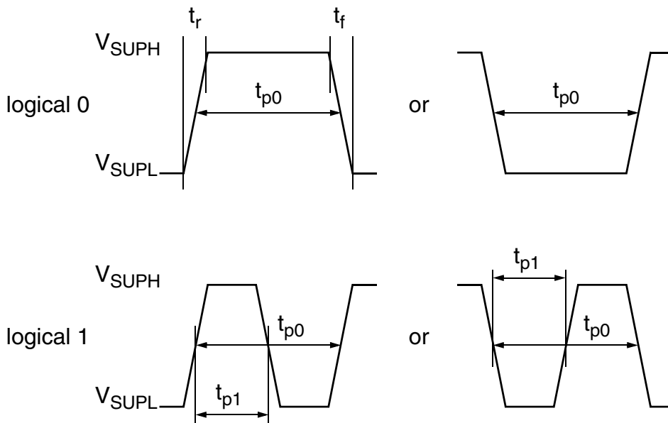
Fig. 6–1: Definition of logical 0 and 1 bit
