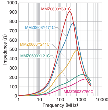
MMZ0603Y series
