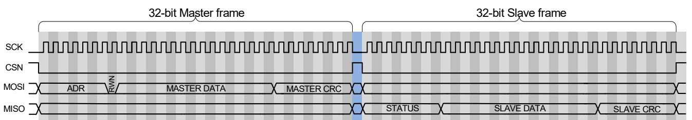
Fig. 7–13: Write command frame structure
