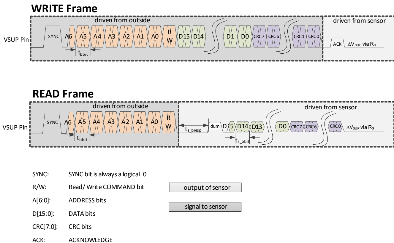
Fig. 10–18: Write and read frames
