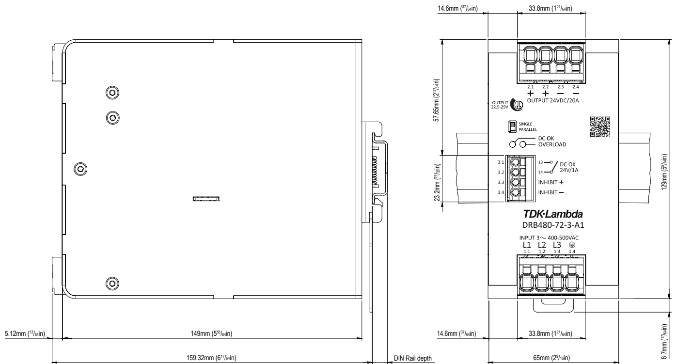
Fig. 19: Dimension drawing of DRB480-72-3-A1
