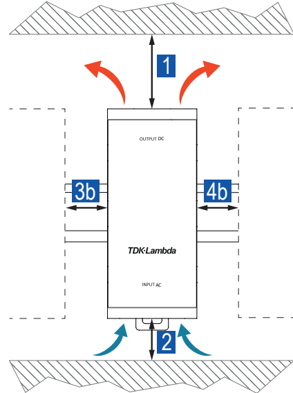
Fig. 21: Installation clearances to passive components
