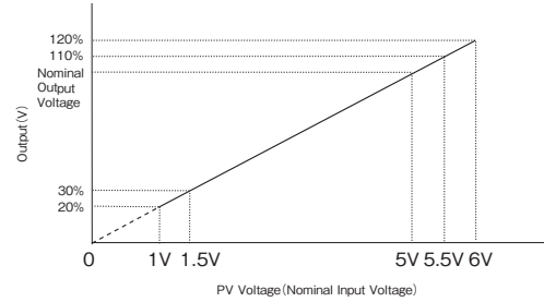
Output Voltage Linearity
