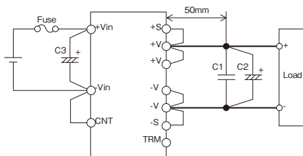
Fig.1-2 Basic Connection
