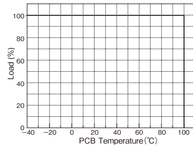
Fig.1-13 Output Derating by PAQ100S48 PCB Temperature
