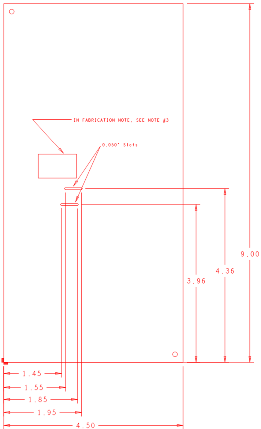
FIGURE 7 Circuit Outline
