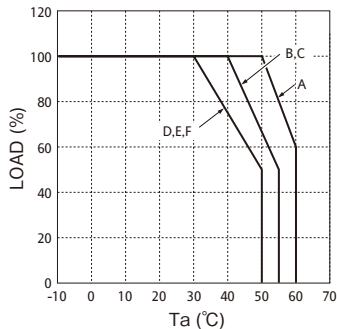
Convection Cooling Output Derating Curve (Without cover)
