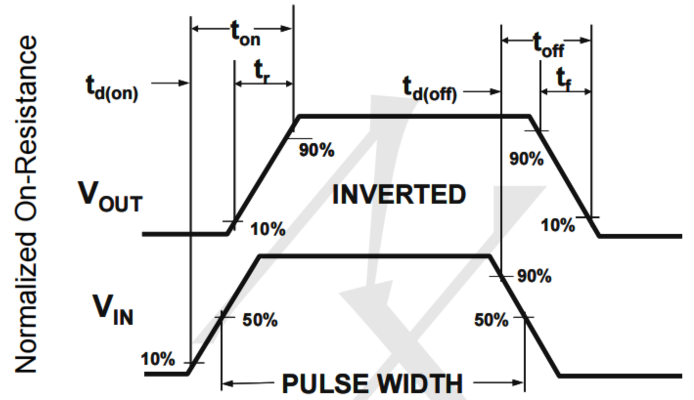
Figure 2: Switching Waveforms
